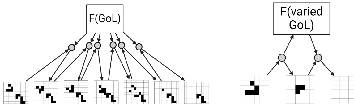
Figure 7: Glider fails to propagate when interacting with the Eater, or with different update rules.
