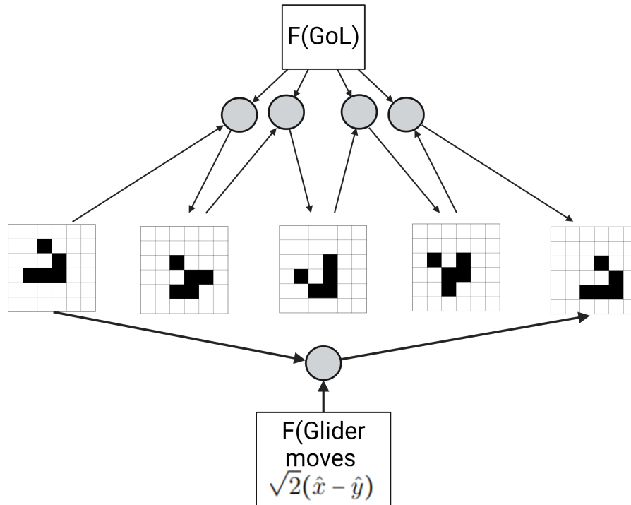
Figure 5: The glider moves \sqrt{2} grid cells every 4 interactions with the f(\text{GoL})
