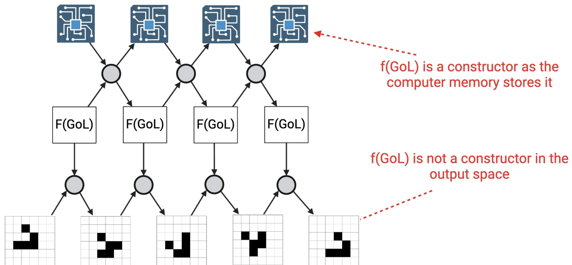
Figure 9: The GoL rules are not constructors, unless we consider the environment of the computer memory and reality.
