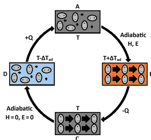
Figure 2: Labelled diagram showing the four cooling stages due to entropy change from the relaxation of the magnetic moments and electric dipoles.
