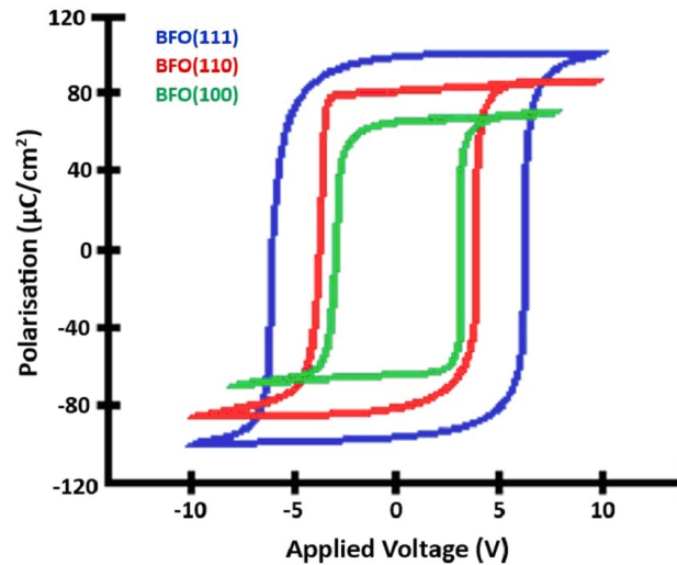
Figure 4: Ferroelectric polarization loops graph for Bismuth Ferrite, \text{BiFeO}_3 based on the data of [6] and [7].
